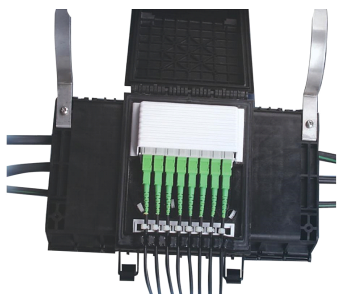
FDC Fiber Optic Splice/Patch Closure, Gel Cable Sealing, 8 SC/APC Adapters, 48 fusion splices
