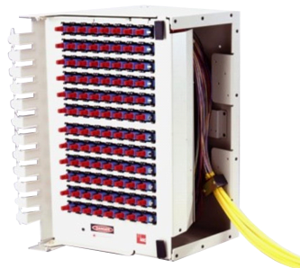
OMX Fiber Termination Block, 96 SC/APC, singlemode, putty white, left oriented
