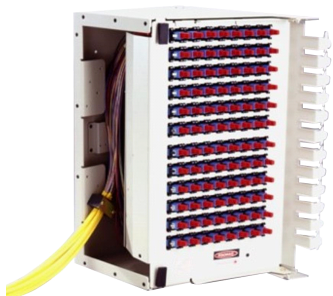
OMX Fiber Termination Block, 96 SC/APC, singlemode, putty white, right oriented
