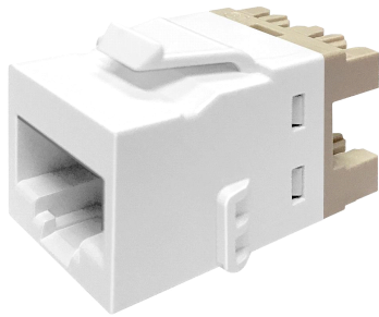
KJ Series Keystone Modular Jack, 8-position, category 6, alpine white
