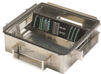
Raised Floor Enclosure, Wide Flange, 24"W x 24"L x 12"D
