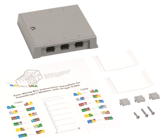
M106 Type Surface Mount Box, six port gray
