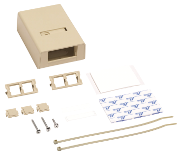
M200 Surface Mount Box, four port ivory
