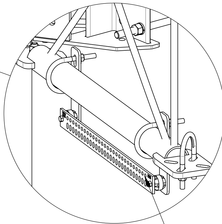
DETAIL E SCALE 1 : 6
