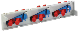
FL2000 Fiber Optic Adapter pack, 3 singlemode SC/UPC duplex adapters
