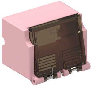
LC Duplex Low Profile Adapter Shutter Assembly, rose with collar with opaque shutter
