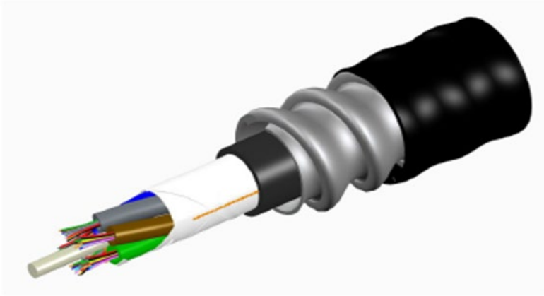
Indoor/Outdoor Riser Rated Aluminum Interlocking Armored Fiber Cable for indoor or outdoor use
